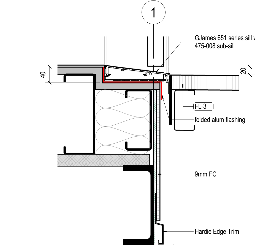
7 North Entry Link - Door Sill 1:5
