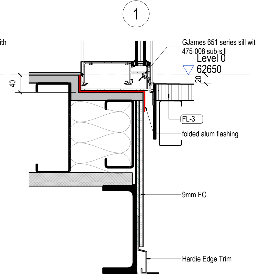
8 North Entry Link - WEF-21 Sill 1:5
