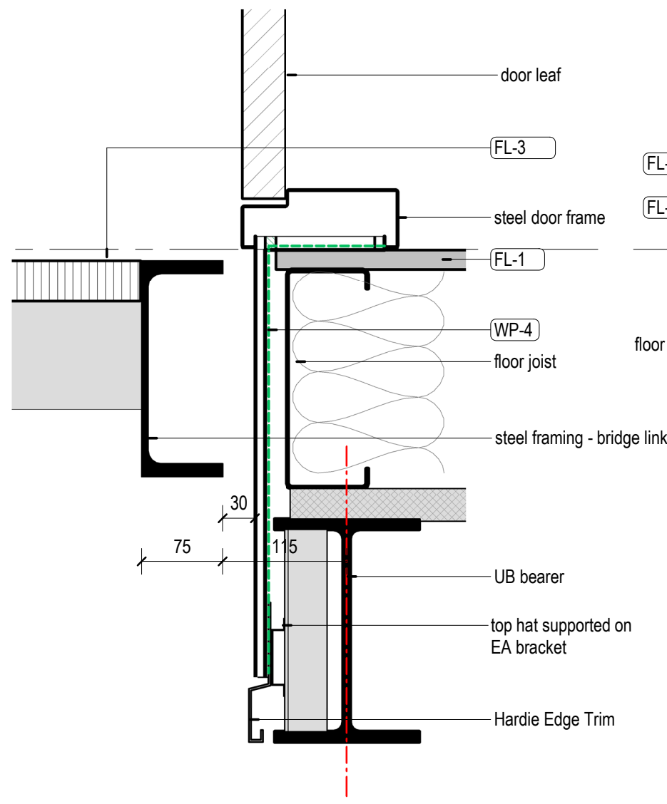
2 West Entry Link - South Edge 1:5
