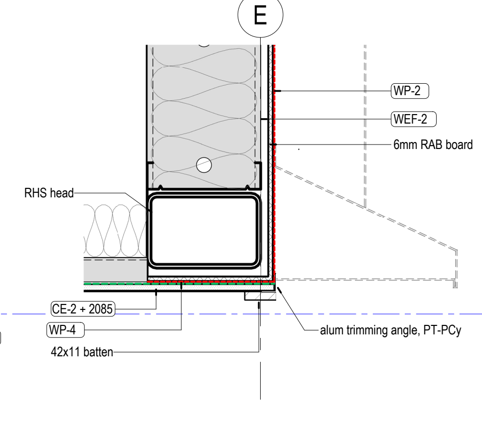
13 East Entry - Facade Ceiling 1:5 Entry Cing Junction
