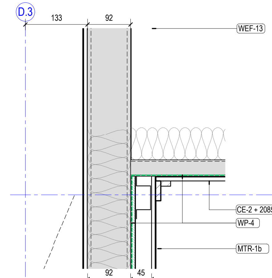
12 East Entry Link - Wall / Ceiling 1:5
