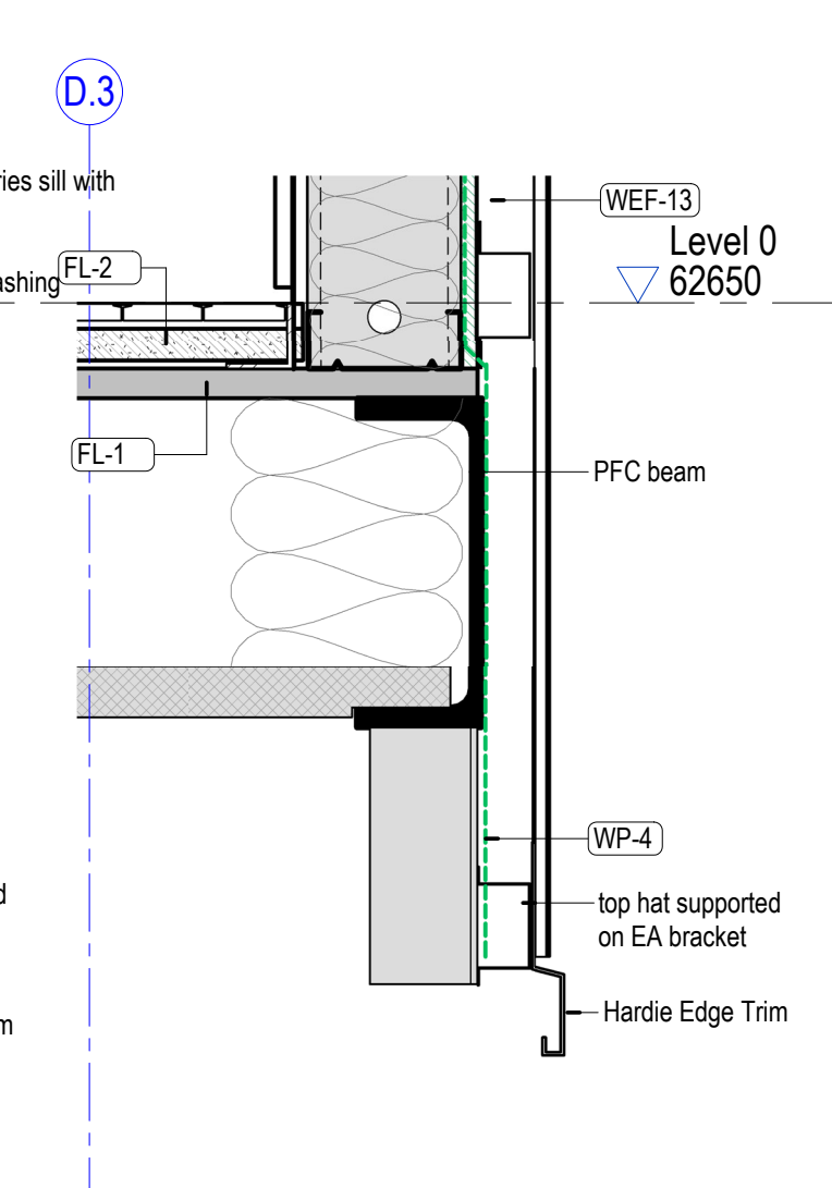
12 East Entry Link - Wall / Ceiling 1:5
