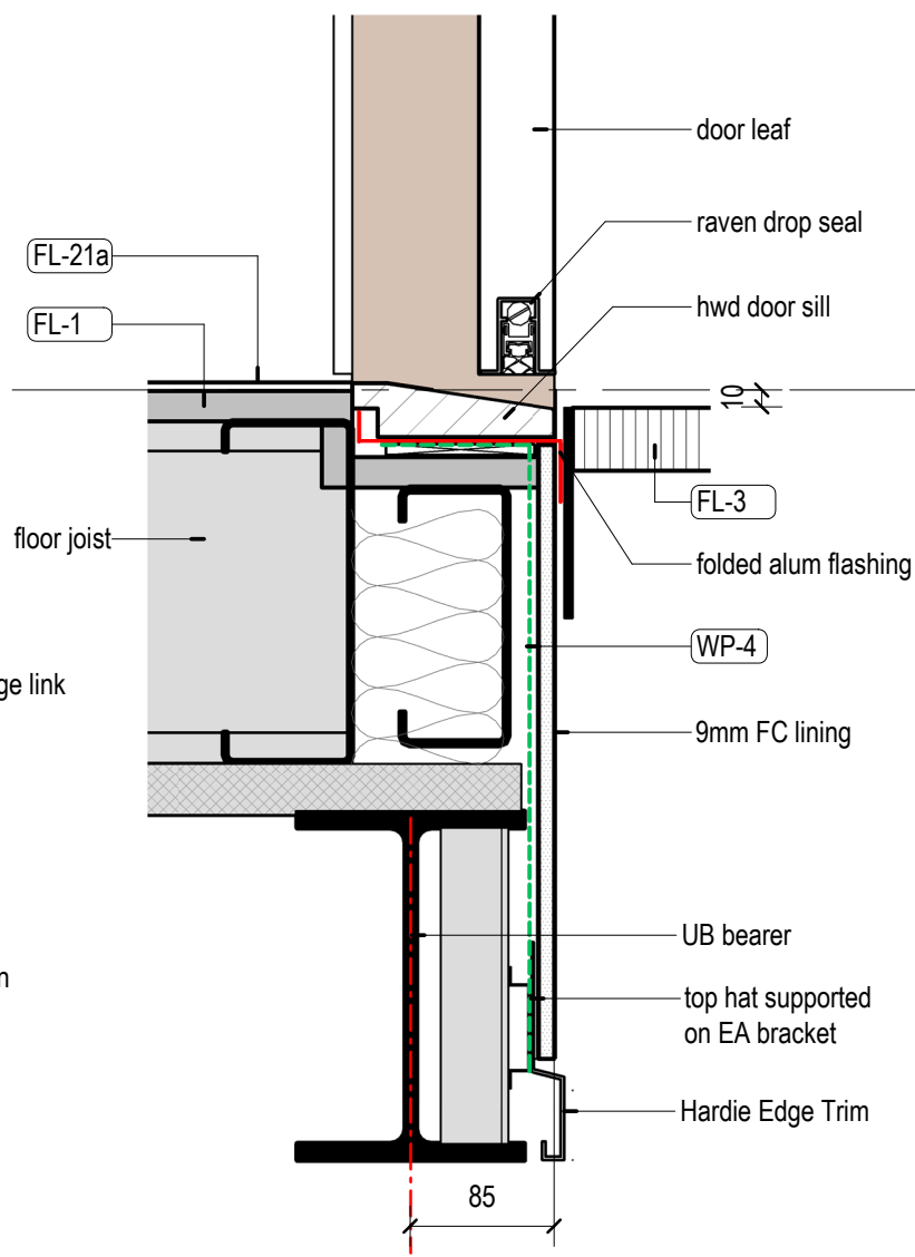
3 West Entry Link - Door Threshold 1:5
