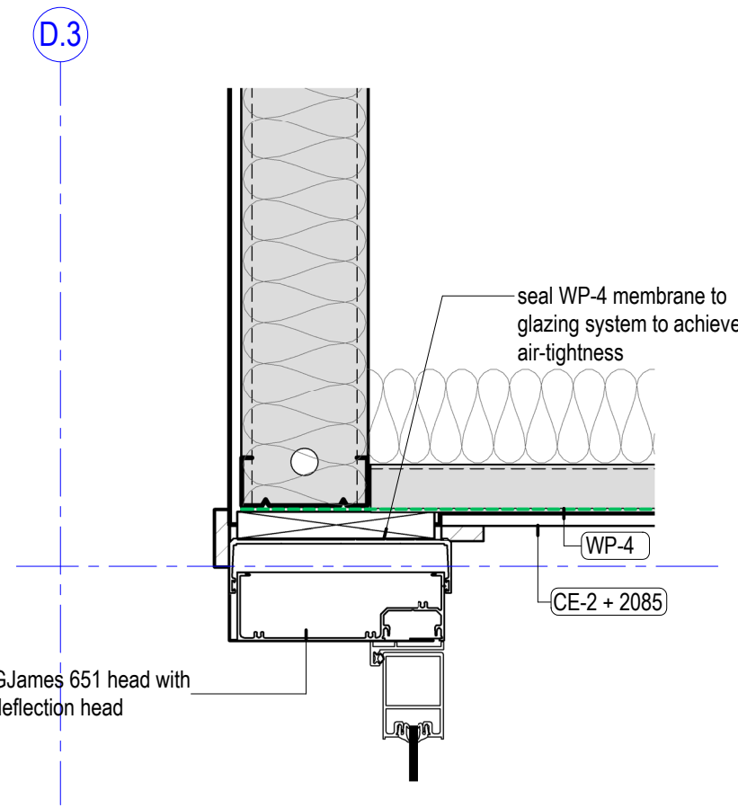
11 East Entry Link - Door Head 1:5
